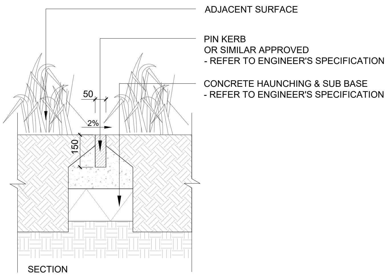
04 TYPICAL DETAIL : PIN KERB SCALE: 1:10 @A1
