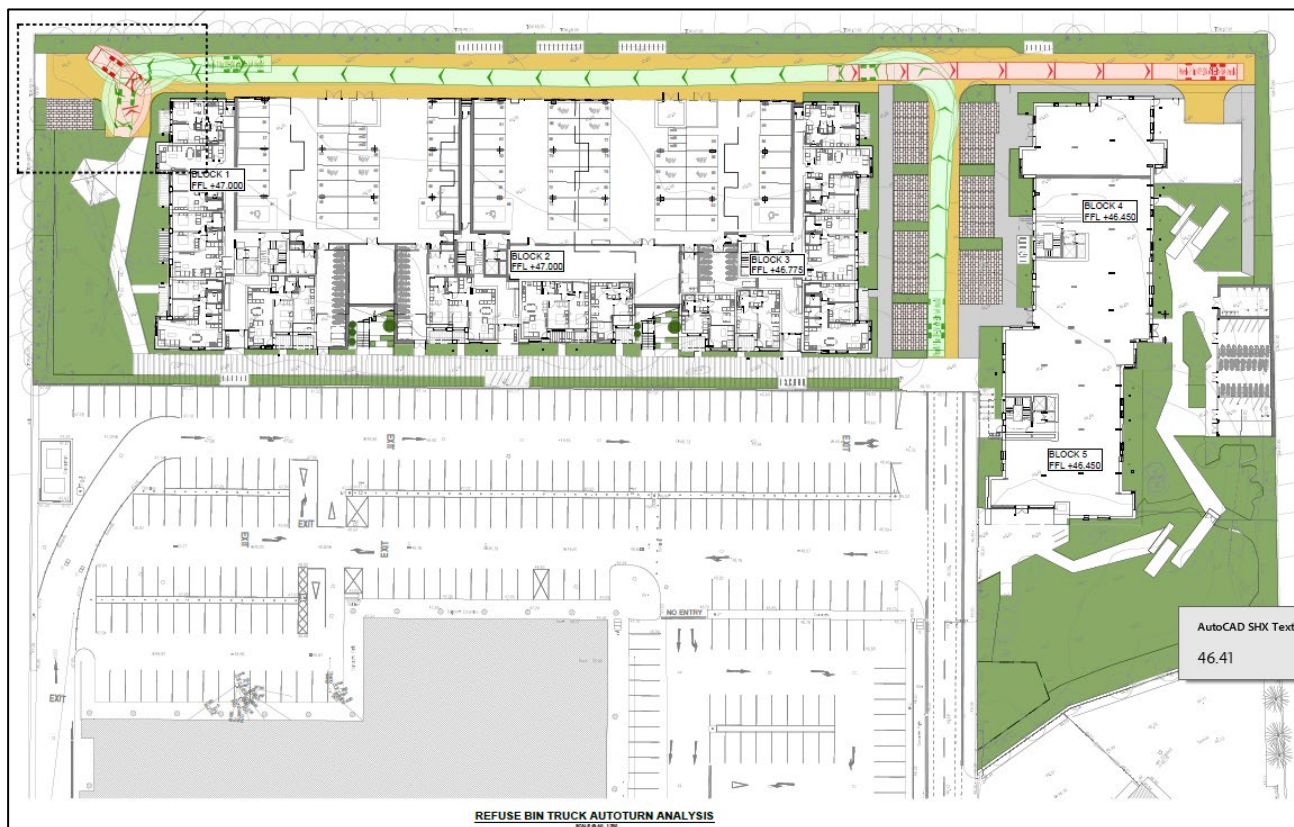
Figure 5.0 Refuse Bin Truck Auto Turn Plan
